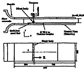
Fig. 1 Schematic diagram of Experimental apparatus
