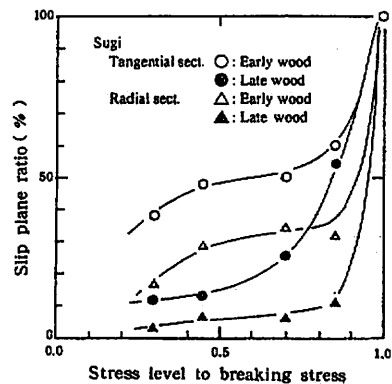
Fig. 2 Percentage of slip planes at various stress level to the slip planes at breaking stress in tangential and radial section 9) (Sugi-wood)
