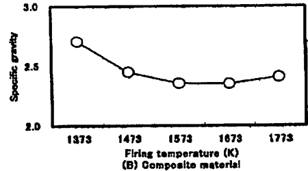
Fig. 2 Comparison of specific gravity when varying the firing temperature
