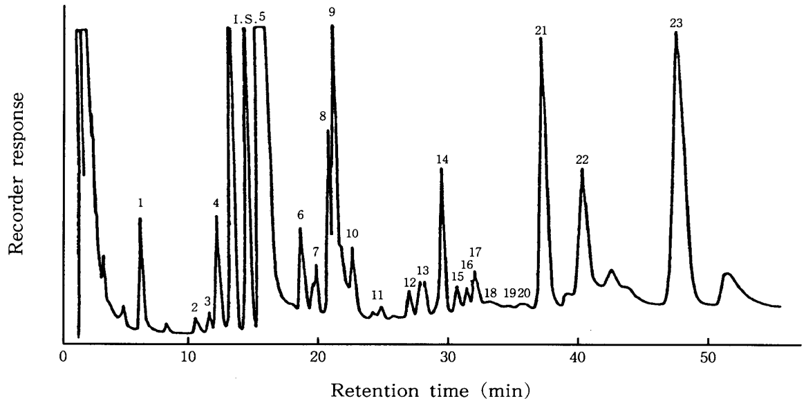
Fig.1. Representative gas chromatogram of aroma concentrate of Kokuto. Identified peaks: (5) 2,3,5-trimethylpyrazine and other pyrazines, (15) 3-hydroxy-2-methyl-pyrone, (22) 2,6-dimethoxyphenol, (23) 4-vinylphenol, (I.S.) internal standard ( n -cyclohexanol).
