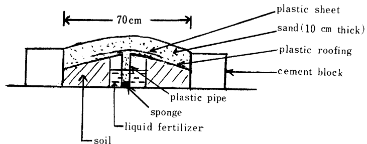
Fig. 1. Diagram of sand bed subirrigated by liquid fertilizer.
